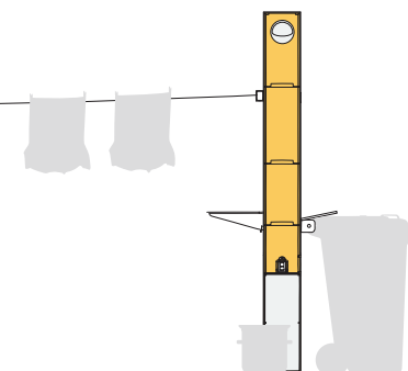
full height, stand alone with Sulo bin holder, tap, drain, power & small table
