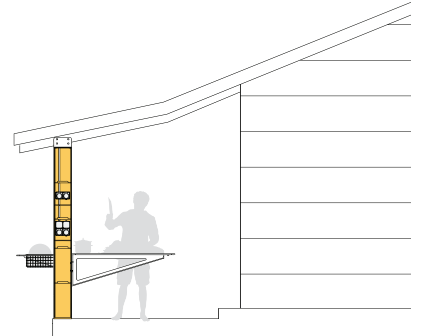
full height, integrated with basket, lights, large table, power & tap
